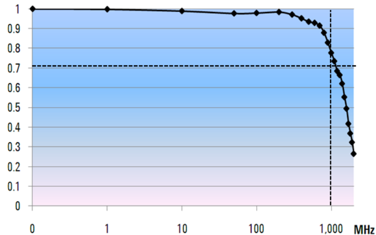
Figure 64 Actual frequency response of an Agilent 1 GHz bandwidth oscilloscope
