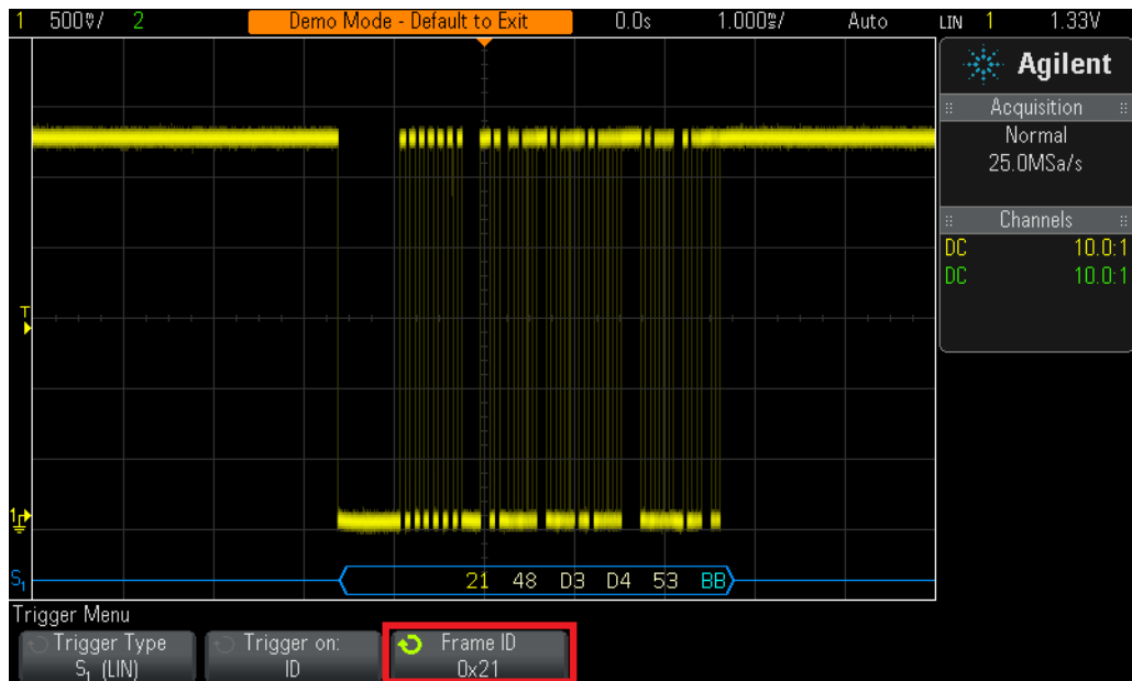
Figure 58 While triggering on LIN frame = 21_{\text{HEX}} , the scope’s hardware-based decoding reveals parity bit errors in the frame ID field.
