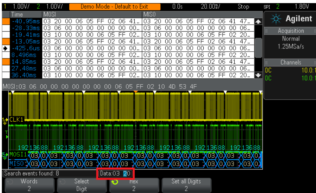
Figure 41 Automatic Search & Navigation on SPI traffic.
