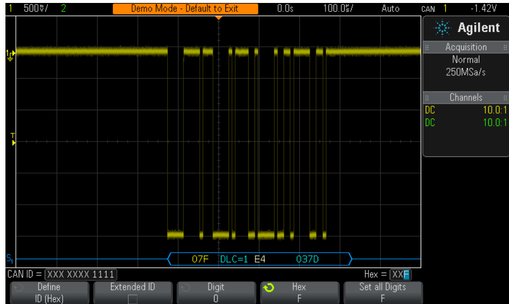
Figure 52 While triggering on CAN data frame = 07F_{\text{HEX}} , the scope’s hardware-based decoding reveals infrequent error conditions.
